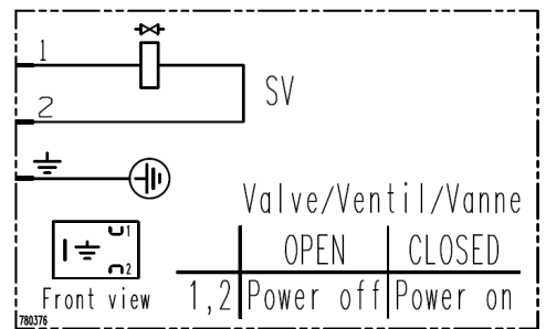
Wiring diagram
