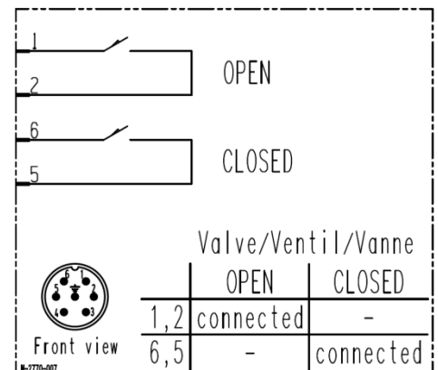
Wiring diagram
