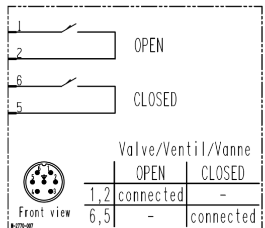
Wiring diagram
