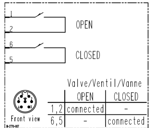
Wiring diagram
