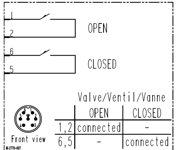
Wiring diagram
