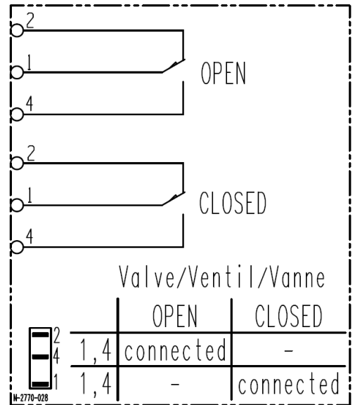
Wiring diagram
