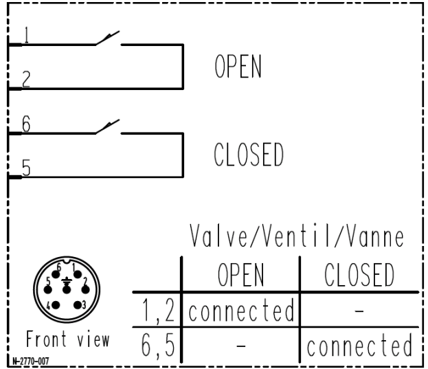
Wiring diagram
