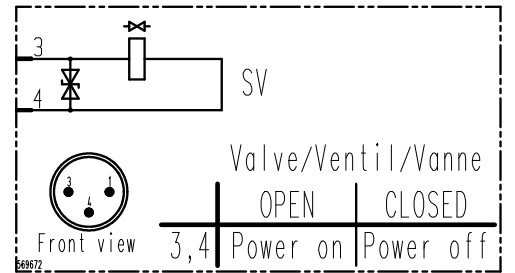
Wiring diagram
