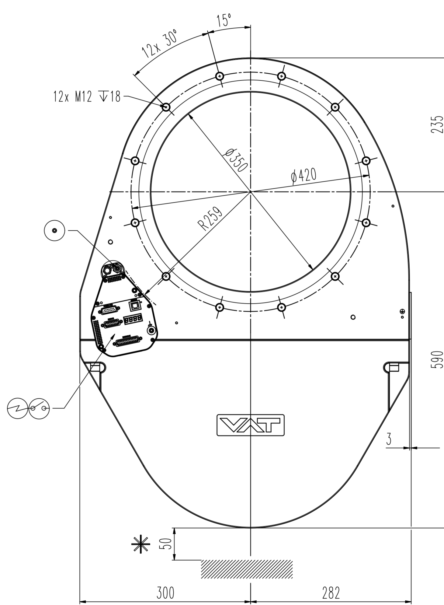
Valve Cluster Slave (without interface)
