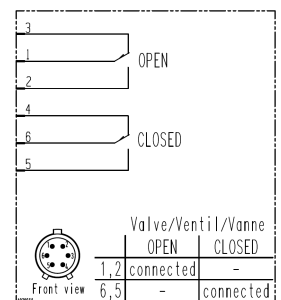
Wiring diagram
