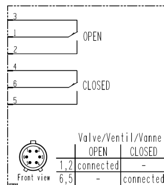
Wiring diagram
