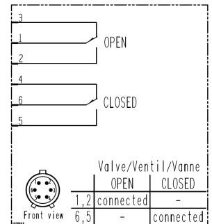
Wiring diagram
