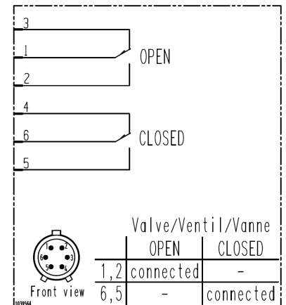
Wiring diagram
