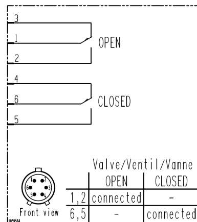
Wiring diagram
