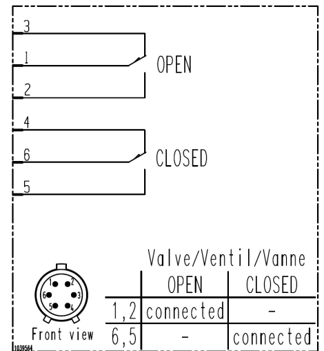
Wiring diagram
