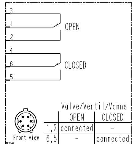
Wiring diagram
