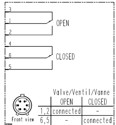
Wiring diagram
